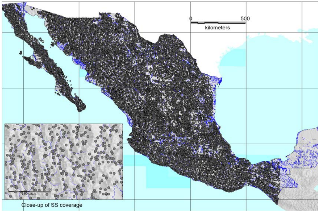
Map showing the area covered by 45,793 stream sediment samples.
